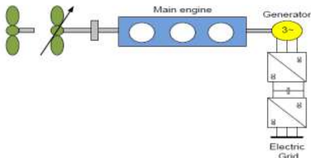
Schematic of PTO/CFE with a slow running generator and conventional or controllable pitch propeller
